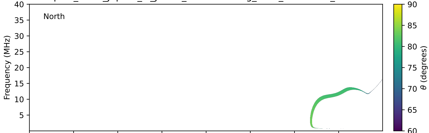
expres_earth_jupiter_io_jrm33_lossc-wid1deg_3kev_19930809_v11.cdf
