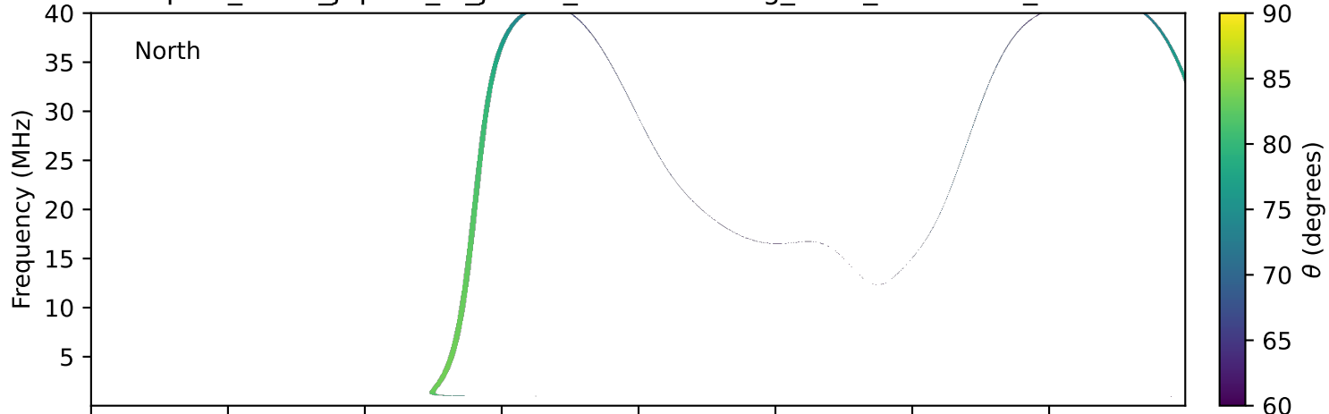
expres_earth_jupiter_io_jrm33_lossc-wid1deg_3kev_19930806_v11.cdf
