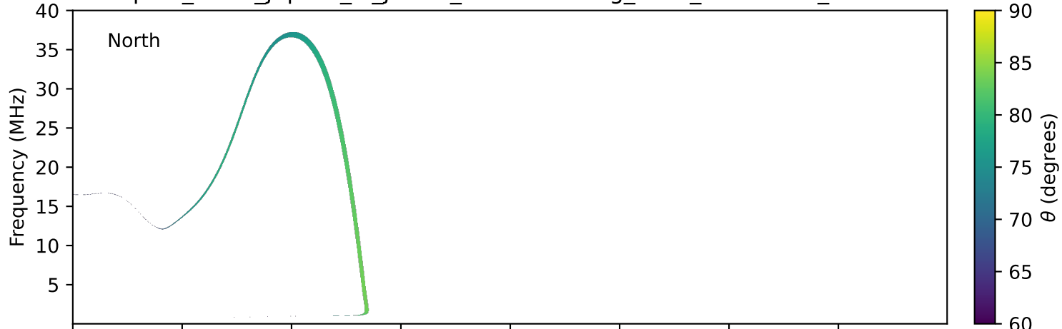
expres_earth_jupiter_io_jrm33_lossc-wid1deg_3kev_19930805_v11.cdf
