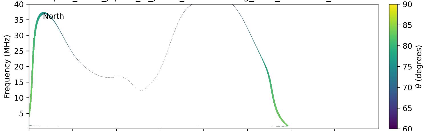
expres_earth_jupiter_io_jrm33_lossc-wid1deg_3kev_19930801_v11.cdf
