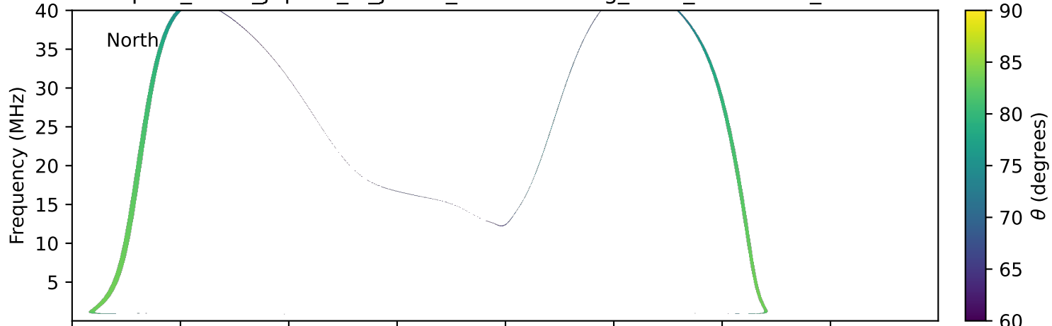
expres_earth_jupiter_io_jrm09_lossc-wid1deg_3kev_19930829_v11.cdf
