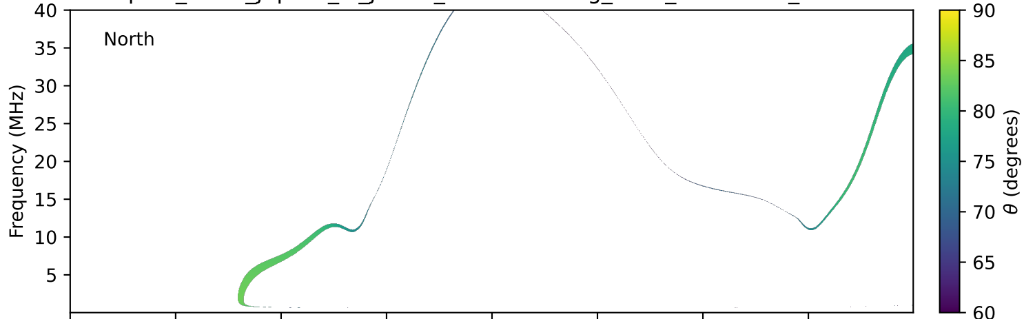
expres_earth_jupiter_io_jrm09_lossc-wid1deg_3kev_19930827_v11.cdf
