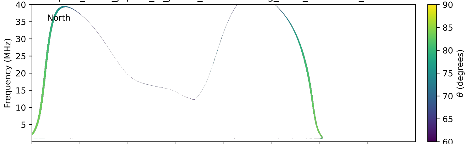
expres_earth_jupiter_io_jrm09_lossc-wid1deg_3kev_19930815_v11.cdf
