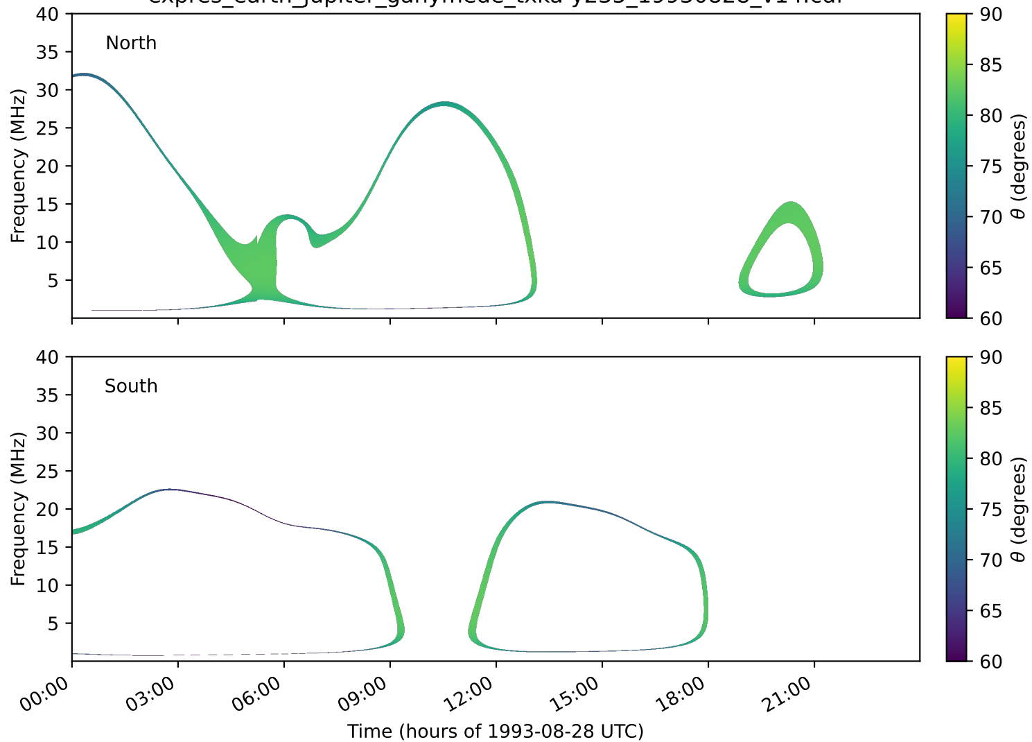
expres_earth_jupiter_ganymede_txka-y235_19930828_v14.cdf
