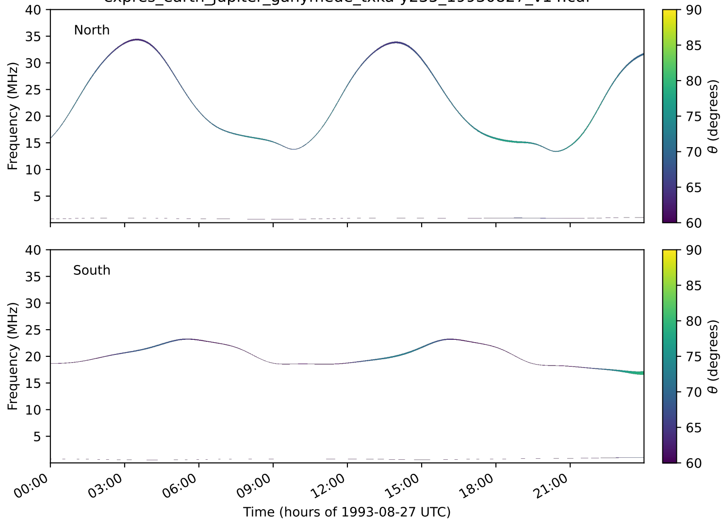
expres_earth_jupiter_ganymede_txka-y235_19930827_v14.cdf
