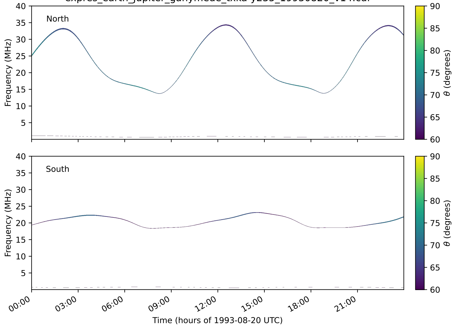
expres_earth_jupiter_ganymede_txka-y235_19930820_v14.cdf
