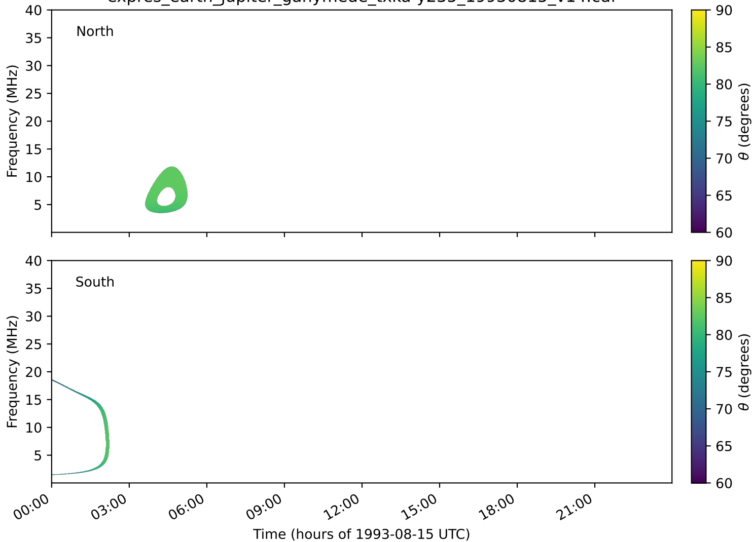
expres_earth_jupiter_ganymede_txka-y235_19930815_v14.cdf
