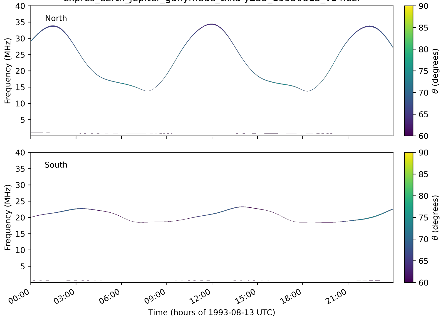
expres_earth_jupiter_ganymede_txka-y235_19930813_v14.cdf
