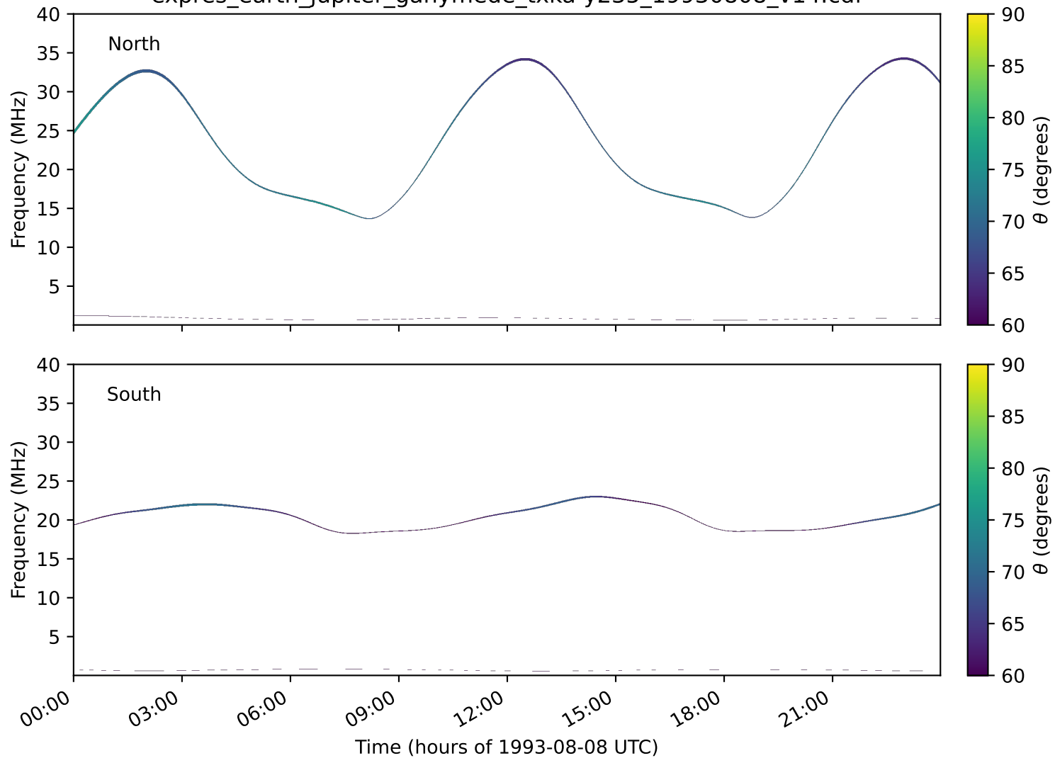
expres_earth_jupiter_ganymede_txka-y235_19930808_v14.cdf
