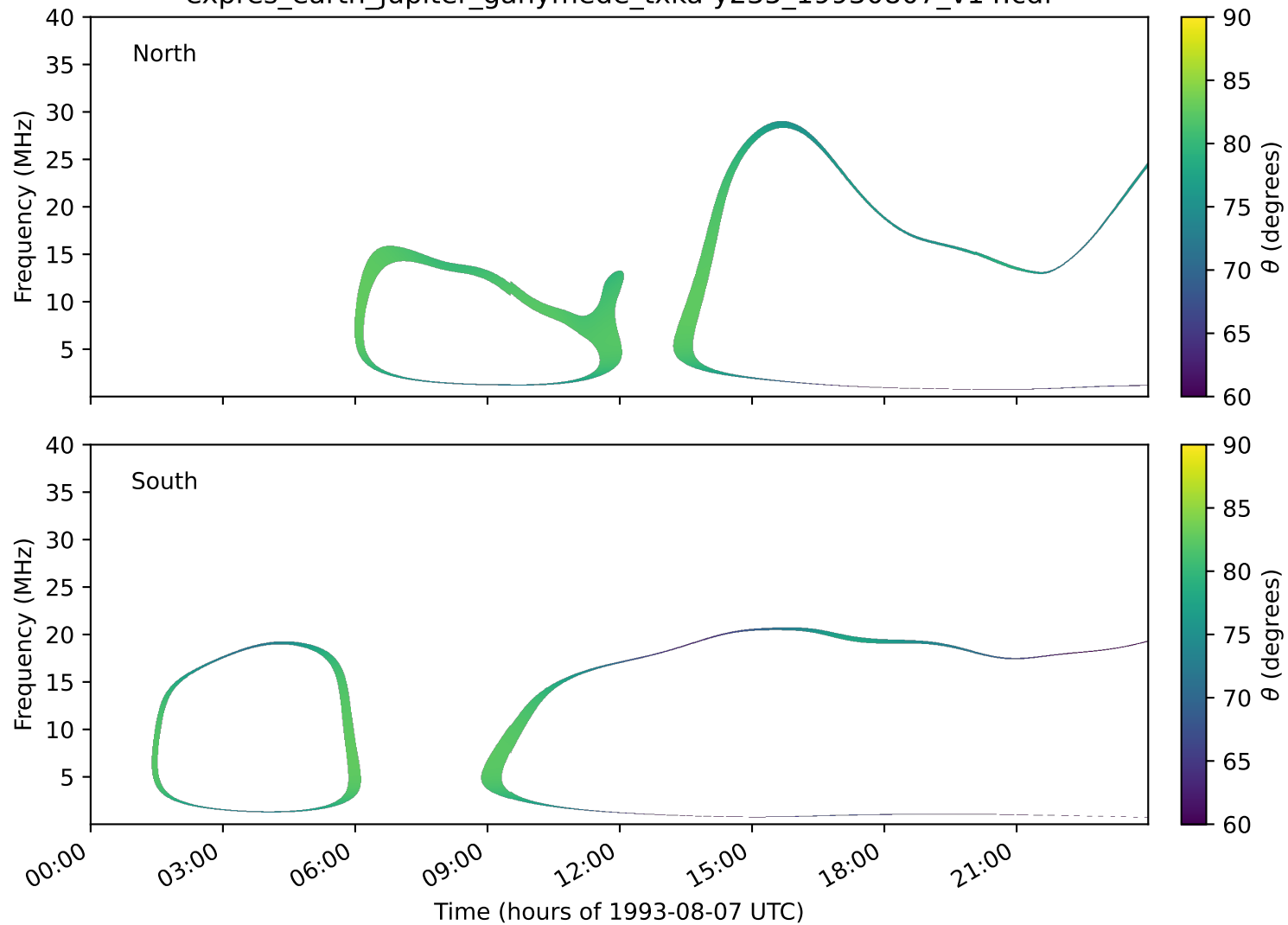
expres_earth_jupiter_ganymede_txka-y235_19930807_v14.cdf
