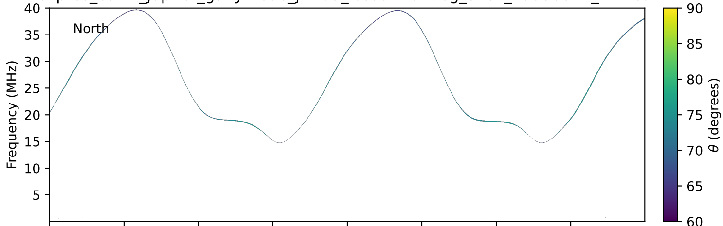
expres_earth_jupiter_ganymede_jrm33_lossc-wid1deg_3kev_19930827_v11.cdf
