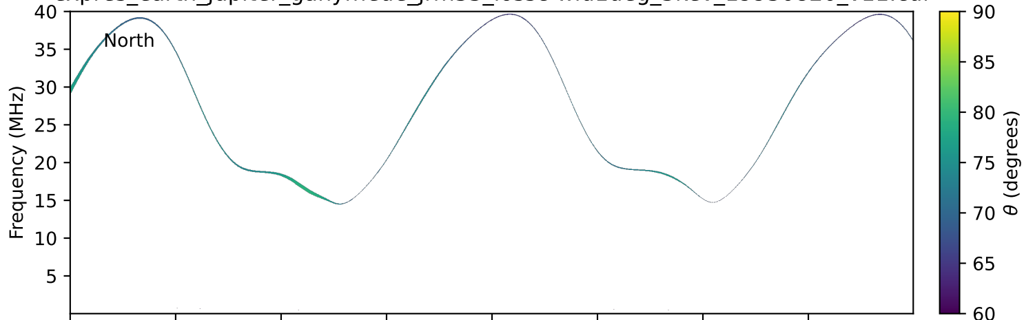
expres_earth_jupiter_ganymede_jrm33_lossc-wid1deg_3kev_19930820_v11.cdf
