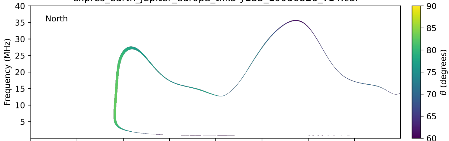
expres_earth_jupiter_europa_txka-y235_19930826_v14.cdf
