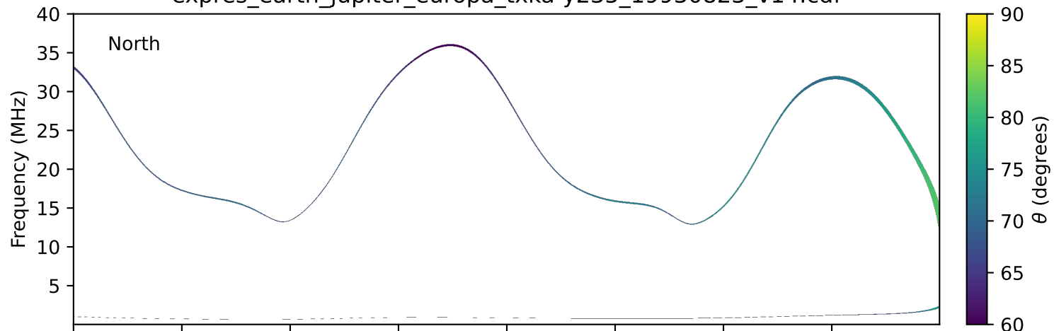
expres_earth_jupiter_europa_txka-y235_19930823_v14.cdf
