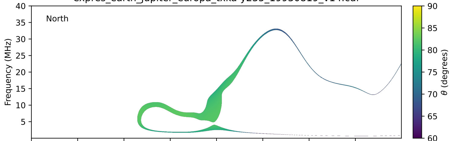
expres_earth_jupiter_europa_txka-y235_19930819_v14.cdf
