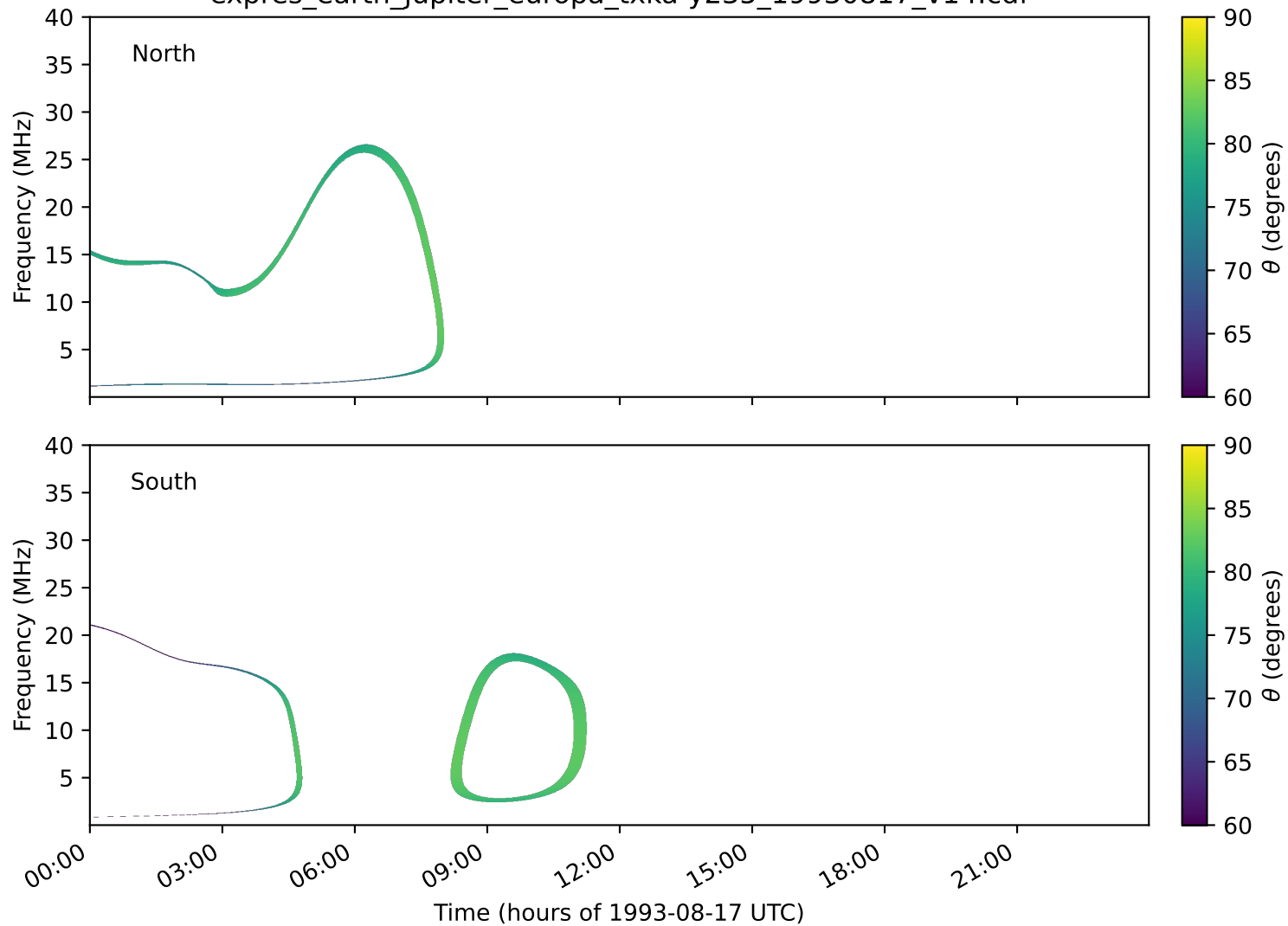
expres_earth_jupiter_europa_txka-y235_19930817_v14.cdf
