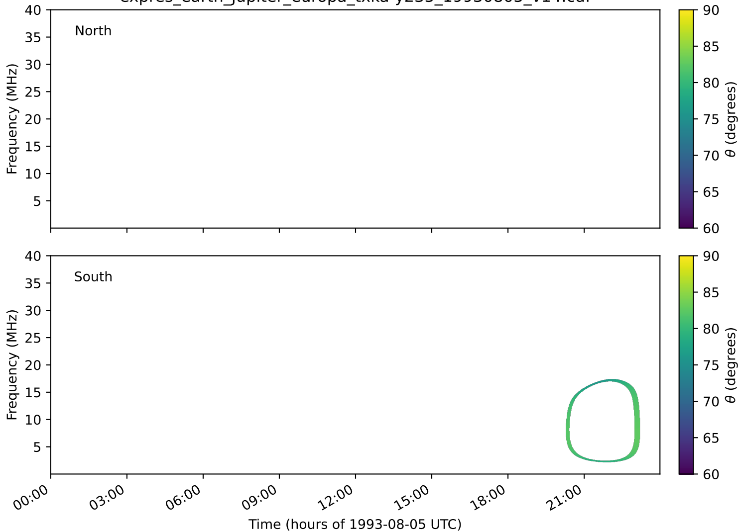
expres_earth_jupiter_europa_txka-y235_19930805_v14.cdf
