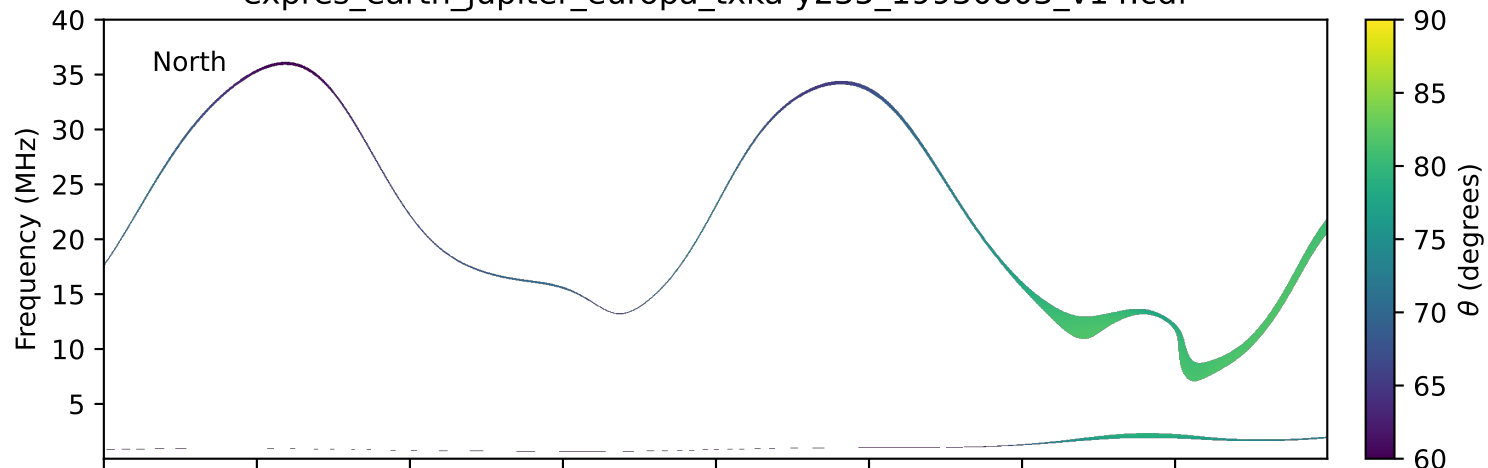
expres_earth_jupiter_europa_txka-y235_19930803_v14.cdf
