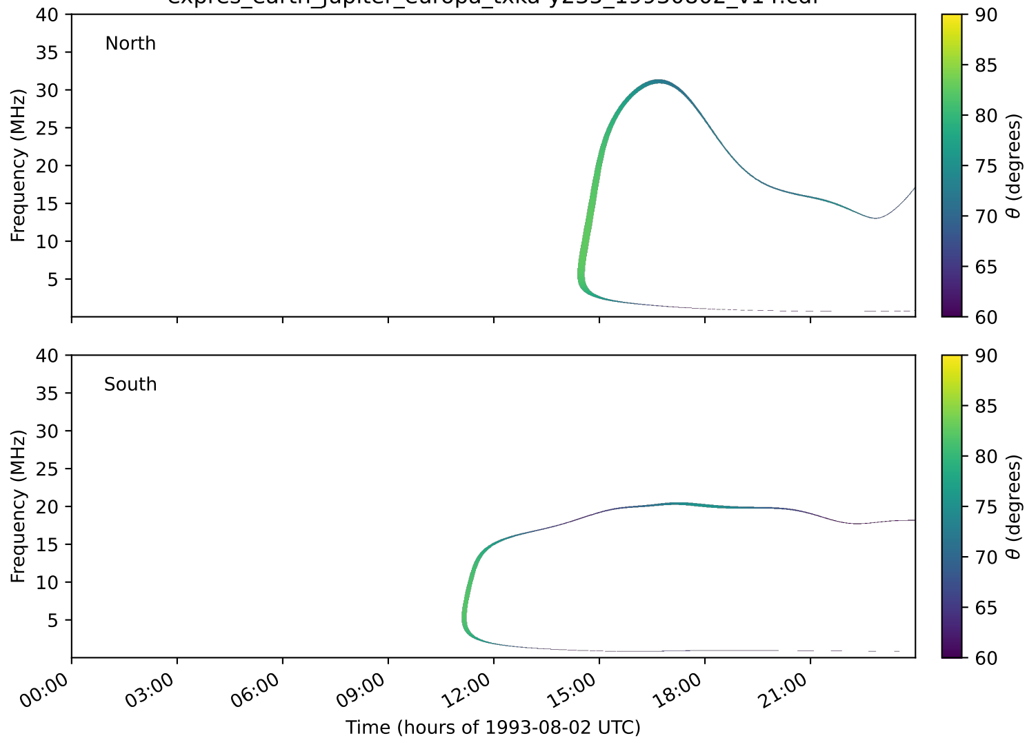
expres_earth_jupiter_europa_txka-y235_19930802_v14.cdf
