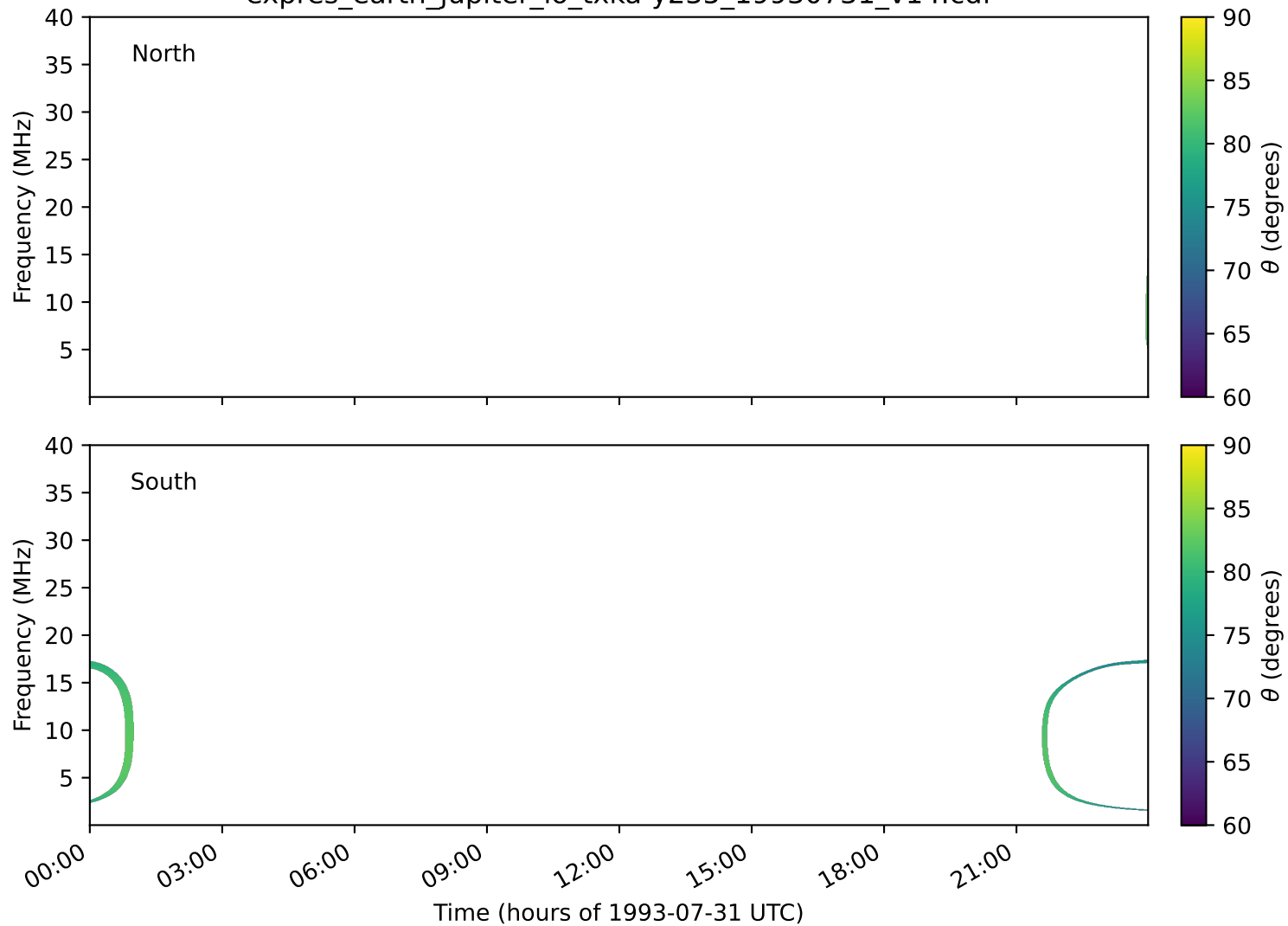
expres_earth_jupiter_io_txka-y235_19930731_v14.cdf
