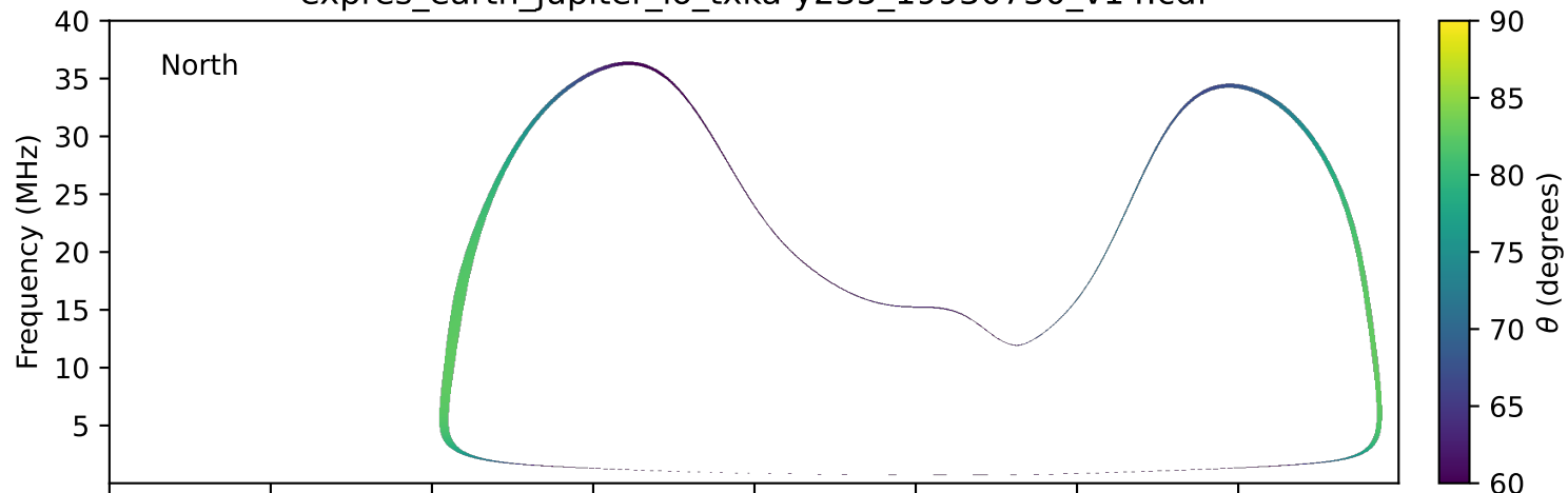
expres_earth_jupiter_io_txka-y235_19930730_v14.cdf
