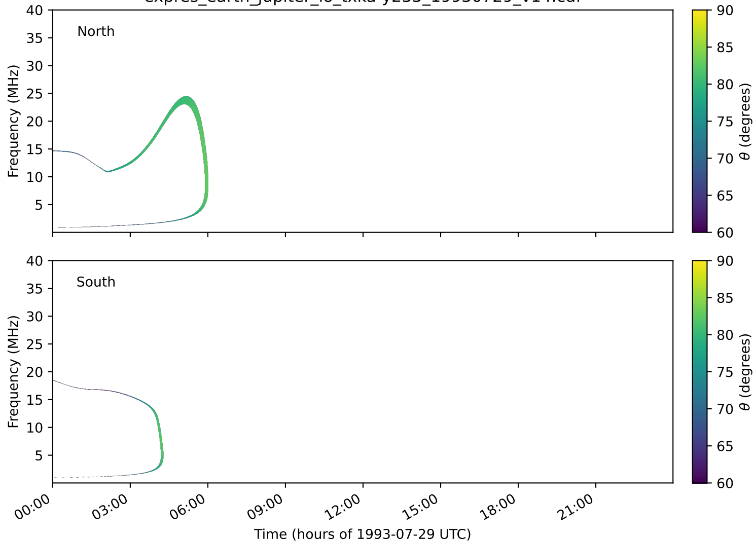
expres_earth_jupiter_io_txka-y235_19930729_v14.cdf
