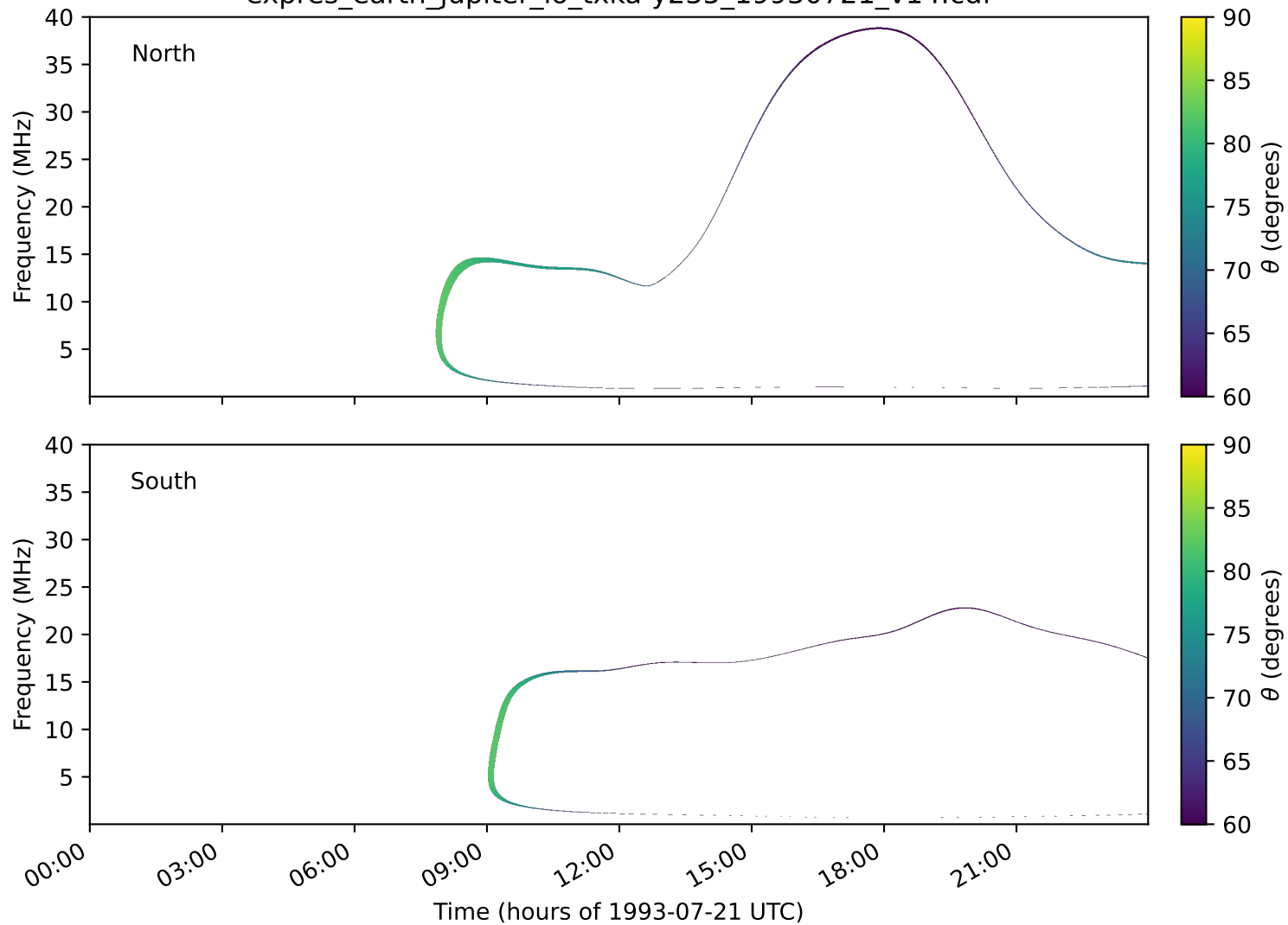
expres_earth_jupiter_io_txka-y235_19930721_v14.cdf
