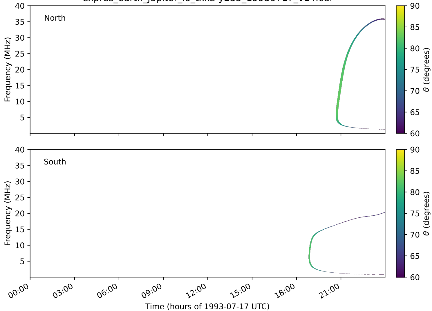
expres_earth_jupiter_io_txka-y235_19930717_v14.cdf
