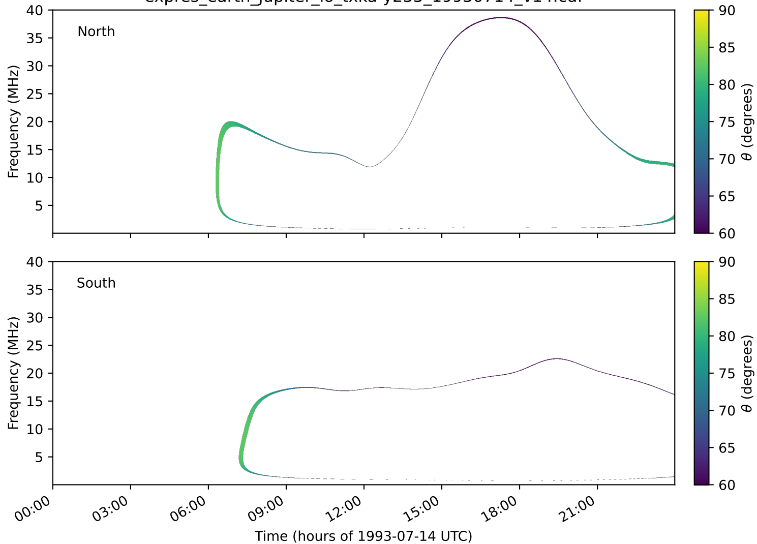
expres_earth_jupiter_io_txka-y235_19930714_v14.cdf
