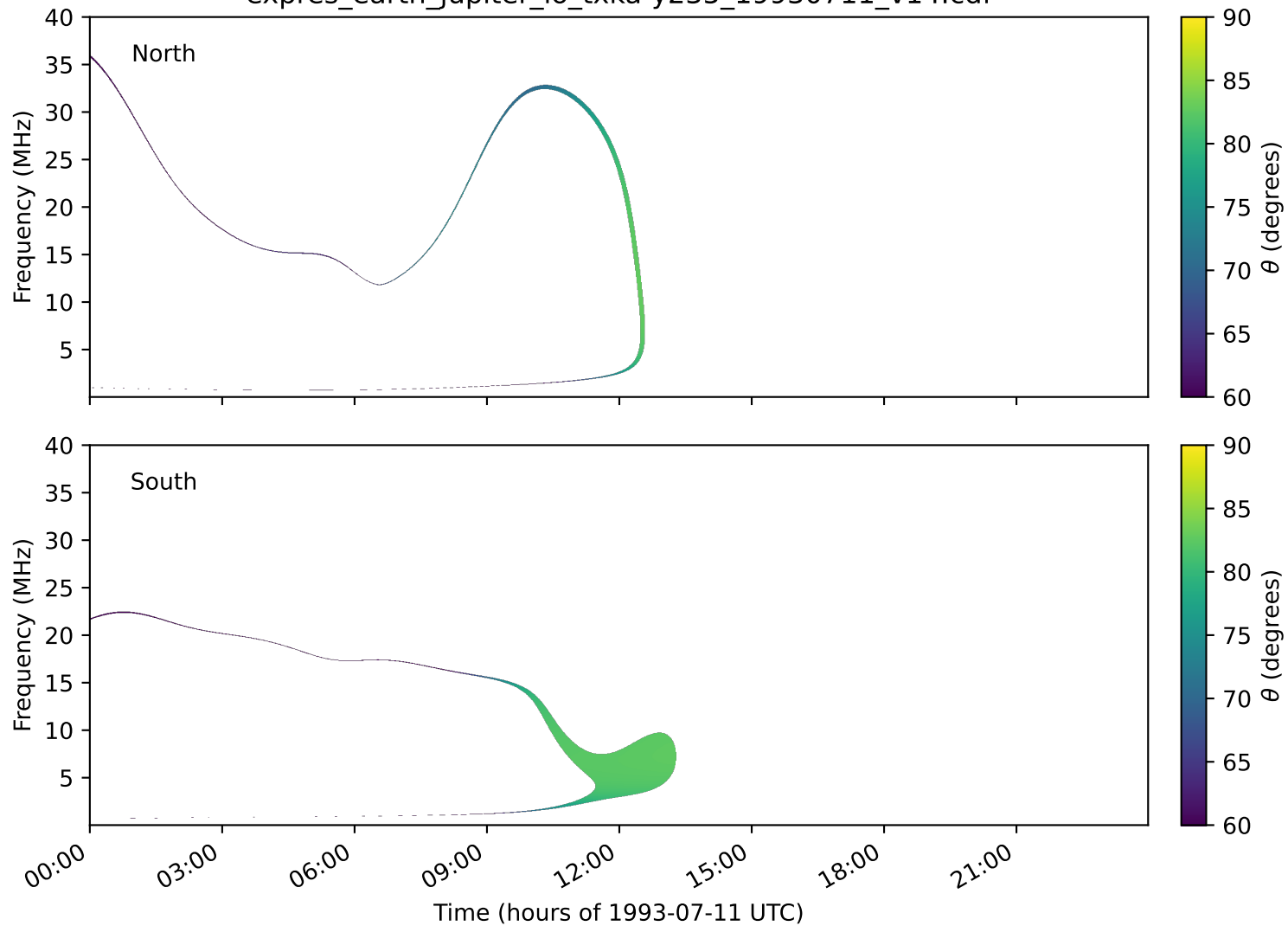
expres_earth_jupiter_io_txka-y235_19930711_v14.cdf
