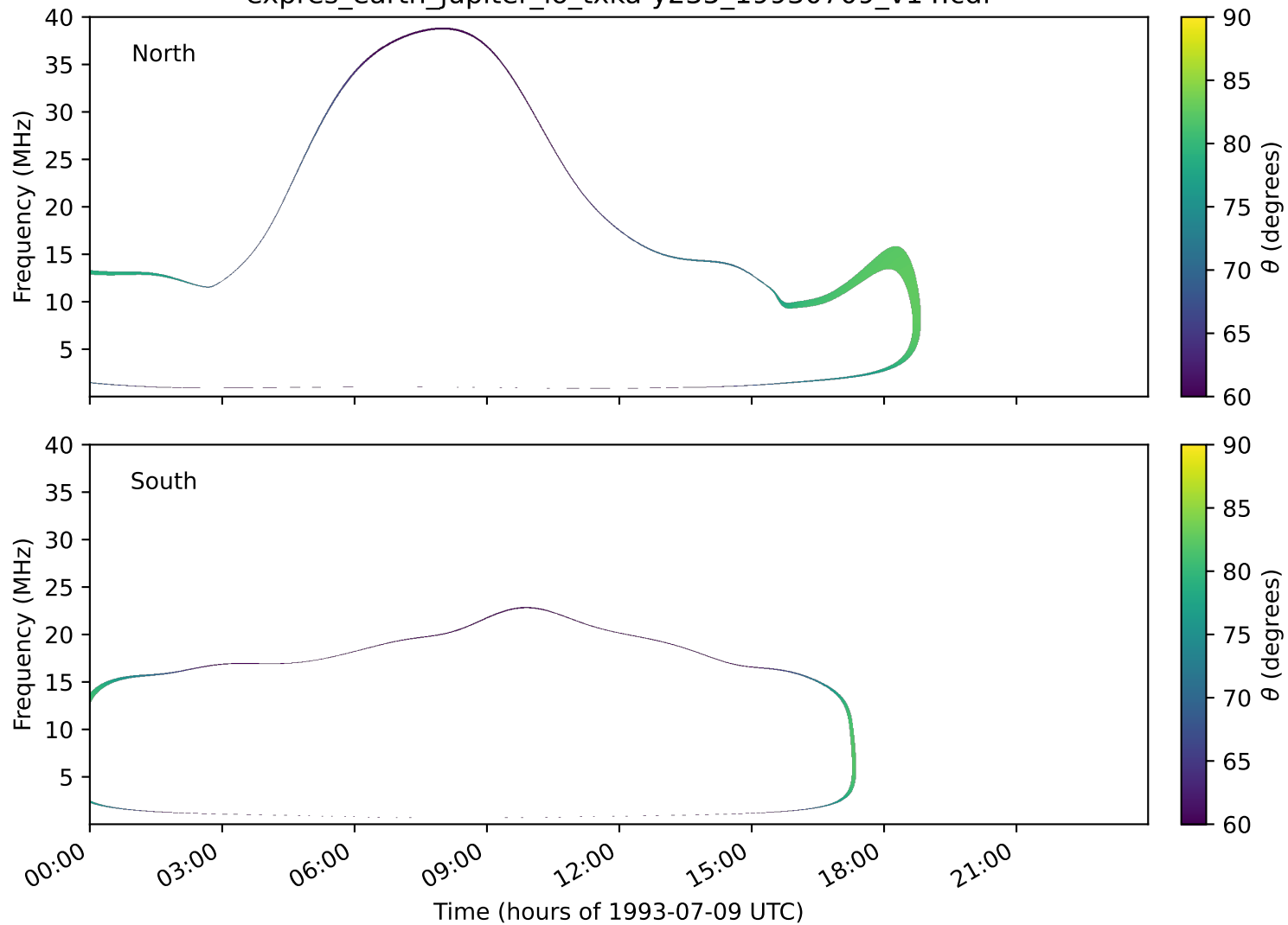
expres_earth_jupiter_io_txka-y235_19930709_v14.cdf
