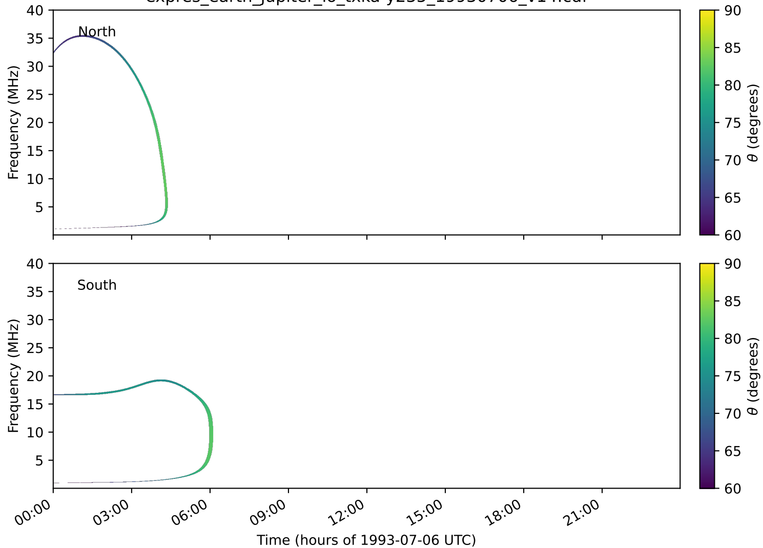
expres_earth_jupiter_io_txka-y235_19930706_v14.cdf
