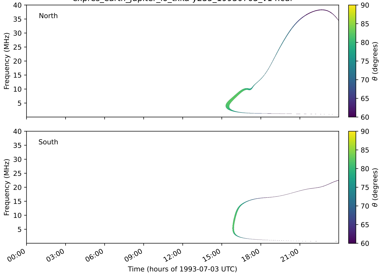
expres_earth_jupiter_io_txka-y235_19930703_v14.cdf
