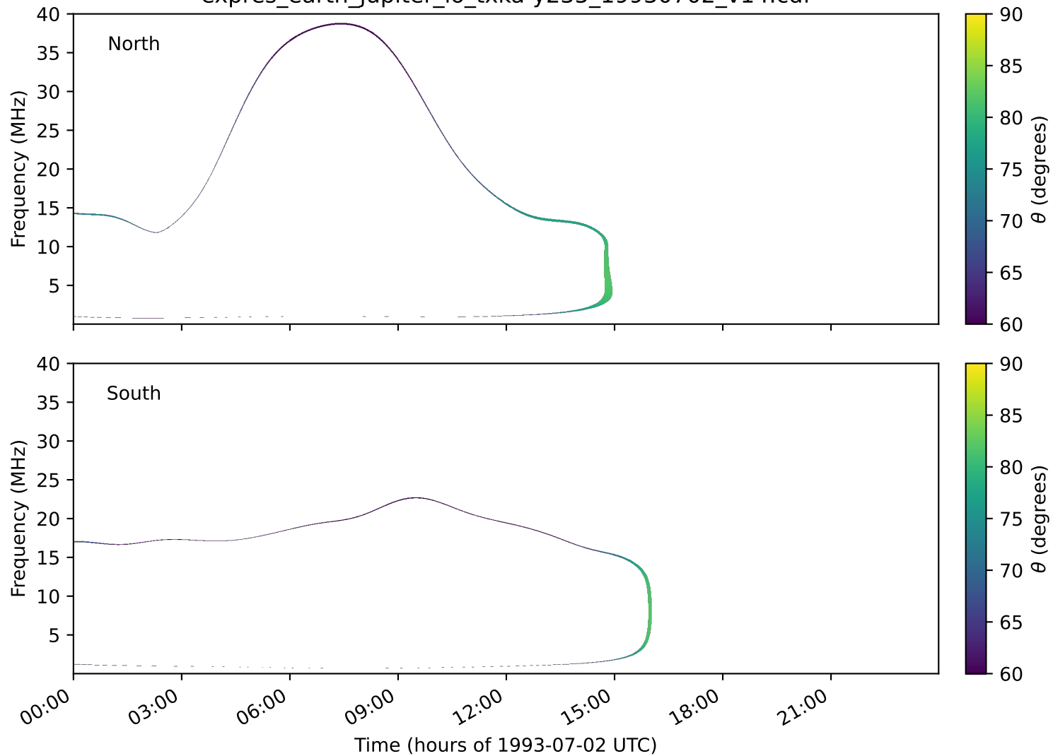
expres_earth_jupiter_io_txka-y235_19930702_v14.cdf
