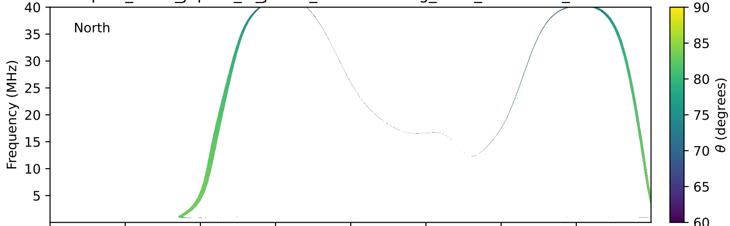
expres_earth_jupiter_io_jrm33_lossc-wid1deg_3kev_19930730_v11.cdf
