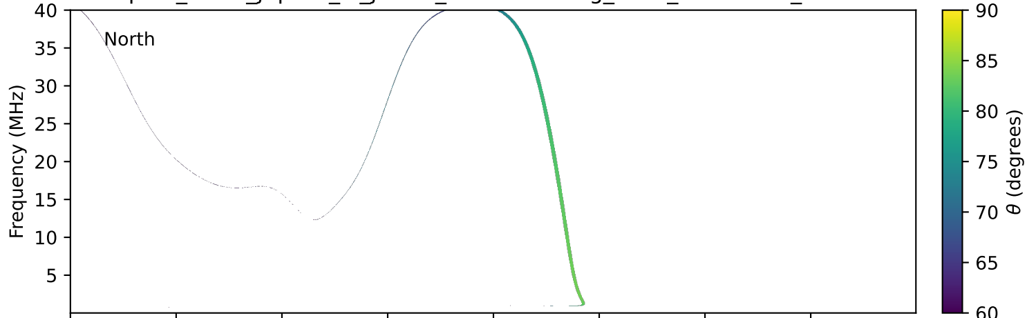
expres_earth_jupiter_io_jrm33_lossc-wid1deg_3kev_19930718_v11.cdf
