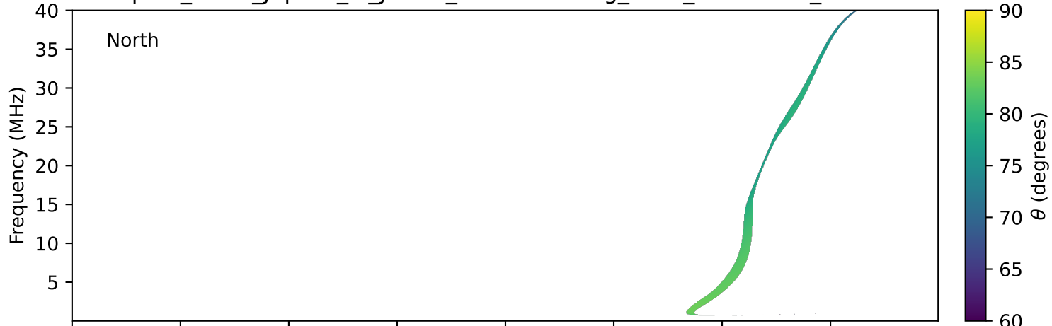
expres_earth_jupiter_io_jrm33_lossc-wid1deg_3kev_19930710_v11.cdf
