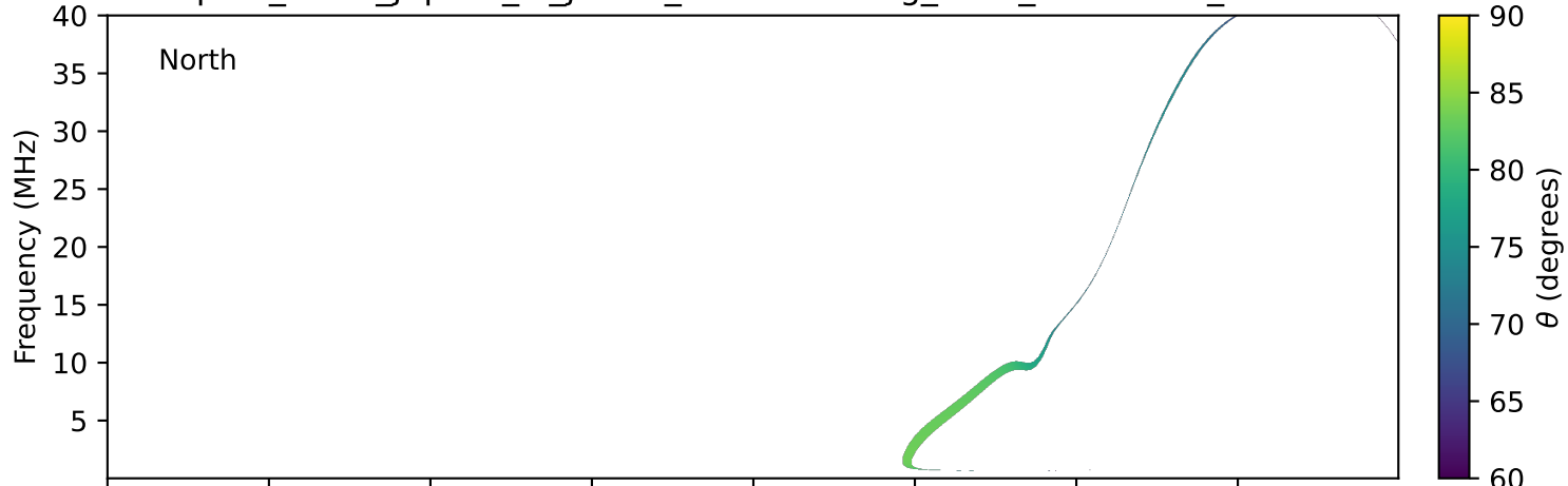
expres_earth_jupiter_io_jrm33_lossc-wid1deg_3kev_19930703_v11.cdf
