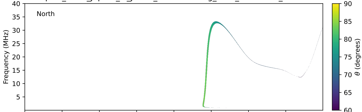
expres_earth_jupiter_io_jrm09_lossc-wid1deg_3kev_19930719_v11.cdf
