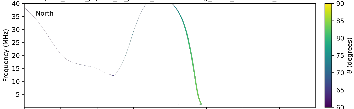
expres_earth_jupiter_io_jrm09_lossc-wid1deg_3kev_19930718_v11.cdf
