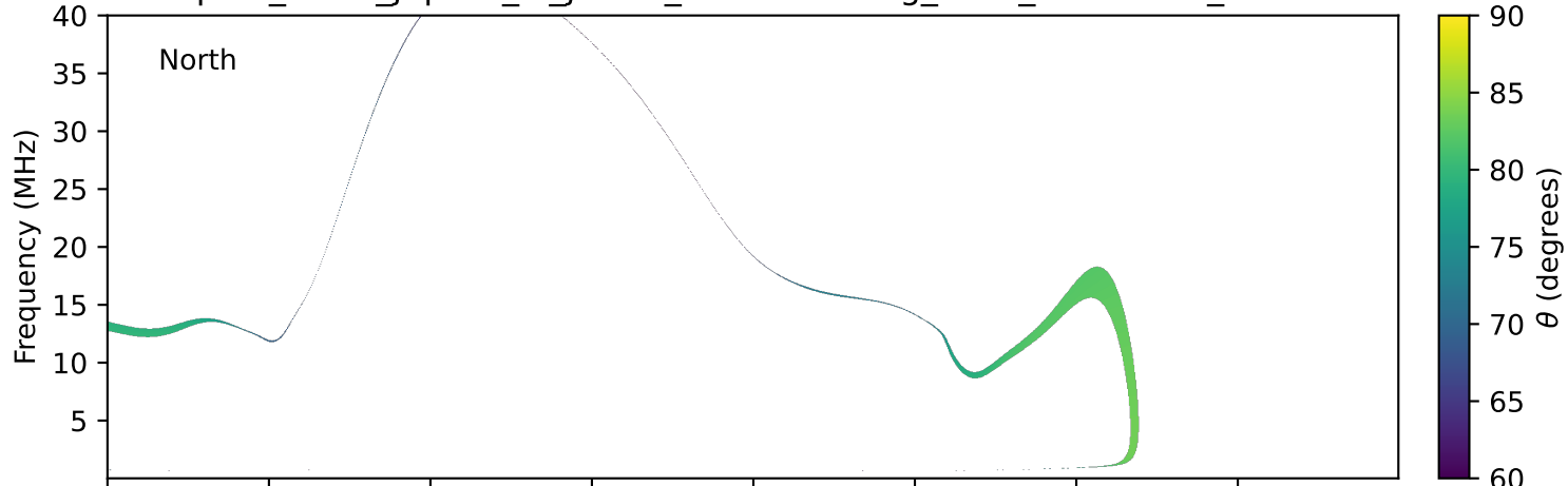
expres_earth_jupiter_io_jrm09_lossc-wid1deg_3kev_19930709_v11.cdf
