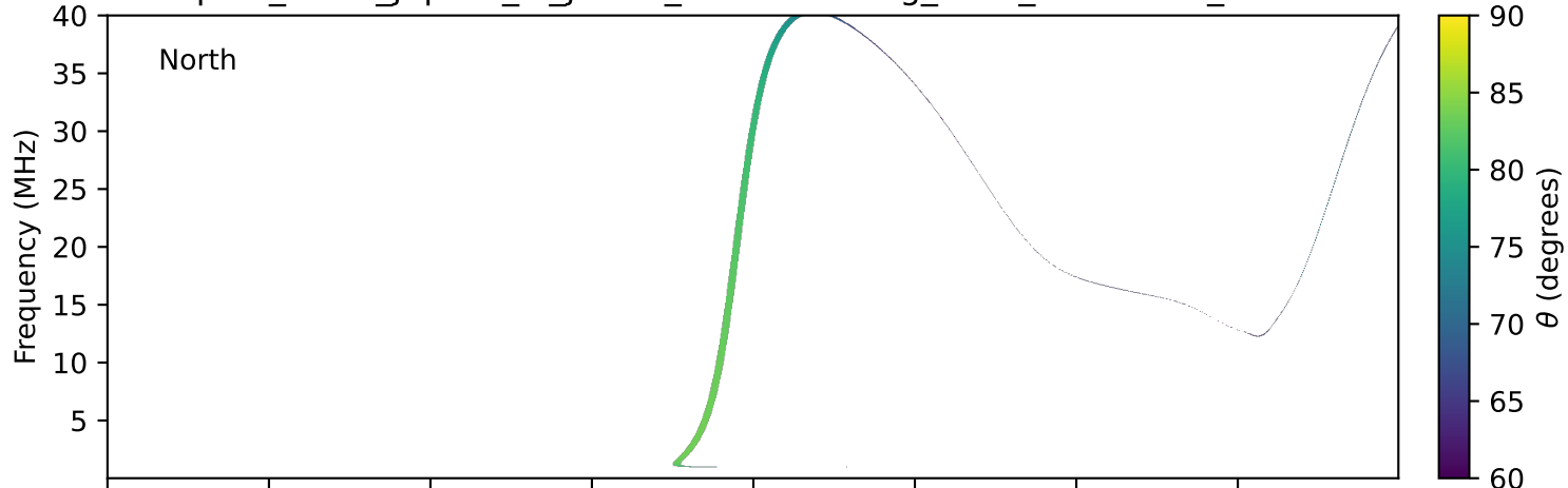
expres_earth_jupiter_io_jrm09_lossc-wid1deg_3kev_19930705_v11.cdf
