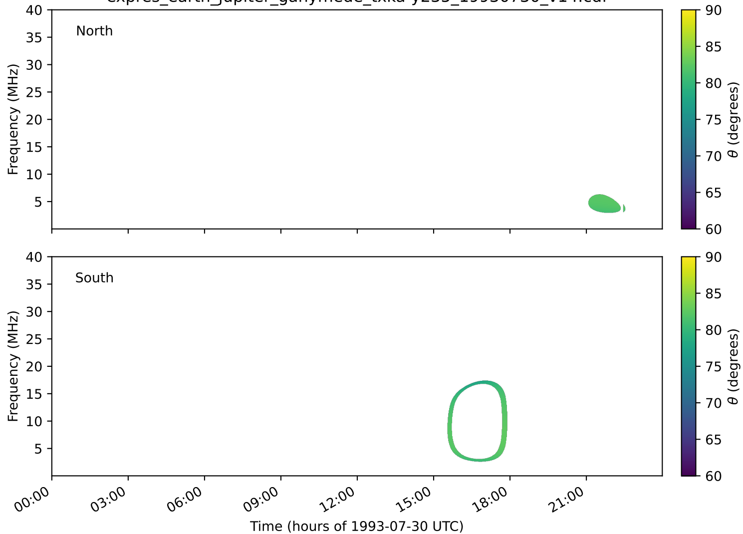
expres_earth_jupiter_ganymede_txka-y235_19930730_v14.cdf
