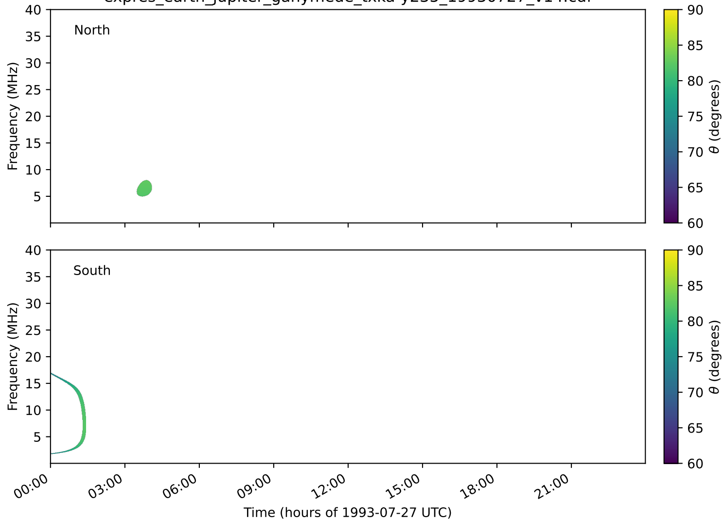
expres_earth_jupiter_ganymede_txka-y235_19930727_v14.cdf
