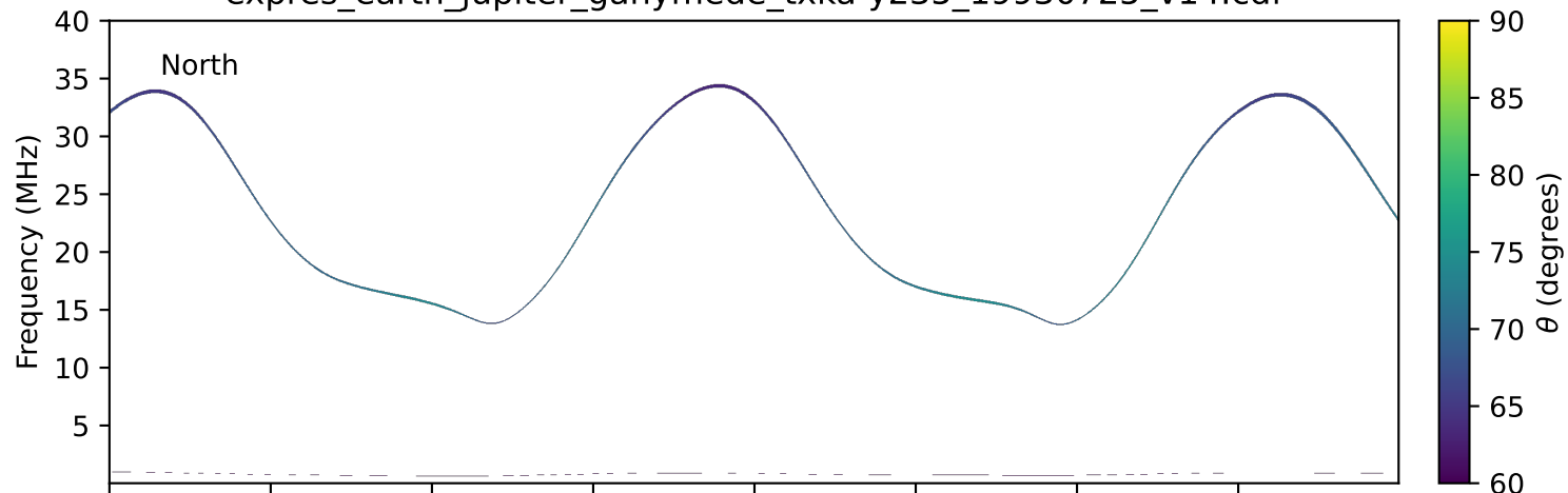
expres_earth_jupiter_ganymede_txka-y235_19930725_v14.cdf
