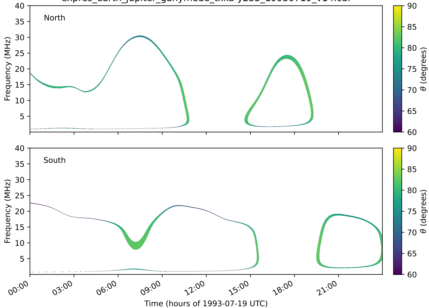
expres_earth_jupiter_ganymede_txka-y235_19930719_v14.cdf
