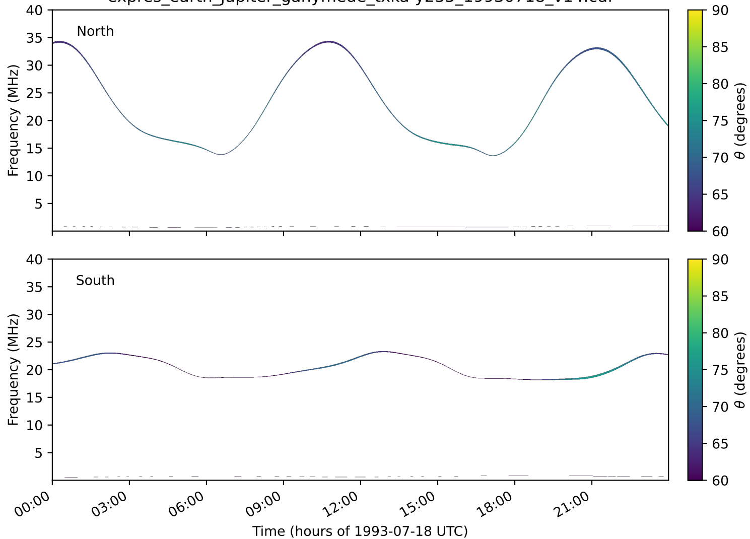
expres_earth_jupiter_ganymede_txka-y235_19930718_v14.cdf
