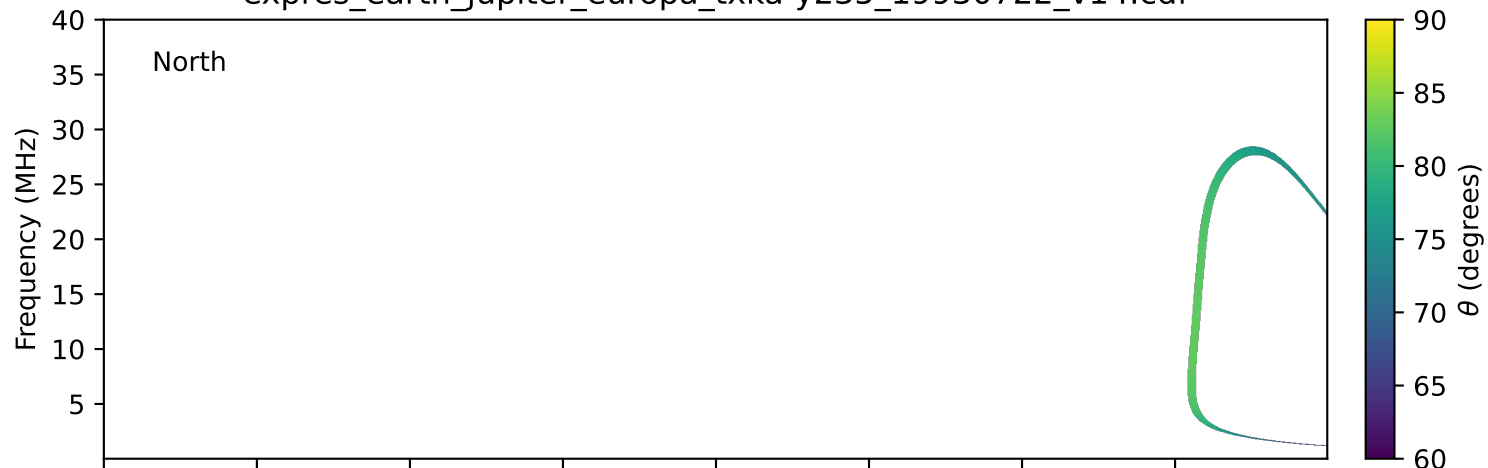
expres_earth_jupiter_europa_txka-y235_19930722_v14.cdf
