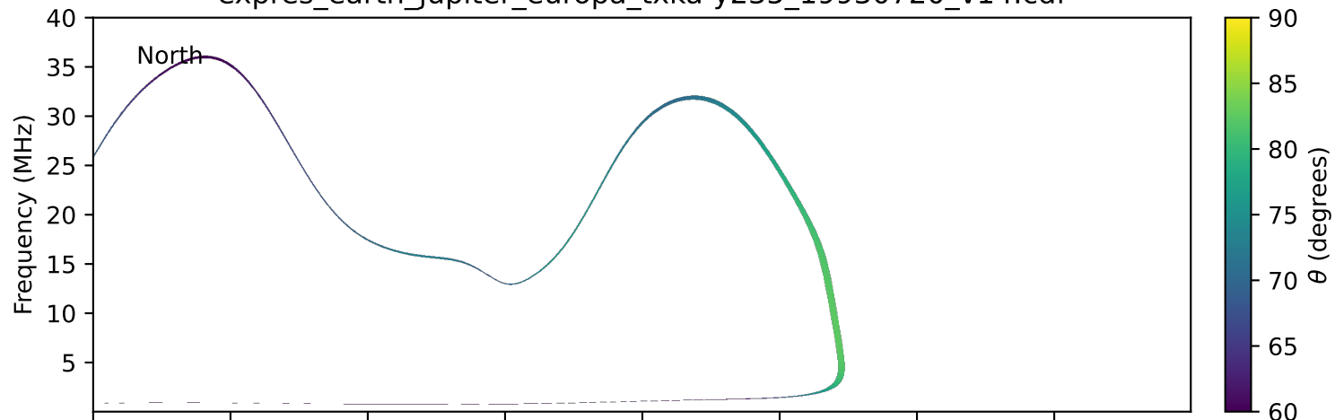
expres_earth_jupiter_europa_txka-y235_19930720_v14.cdf
