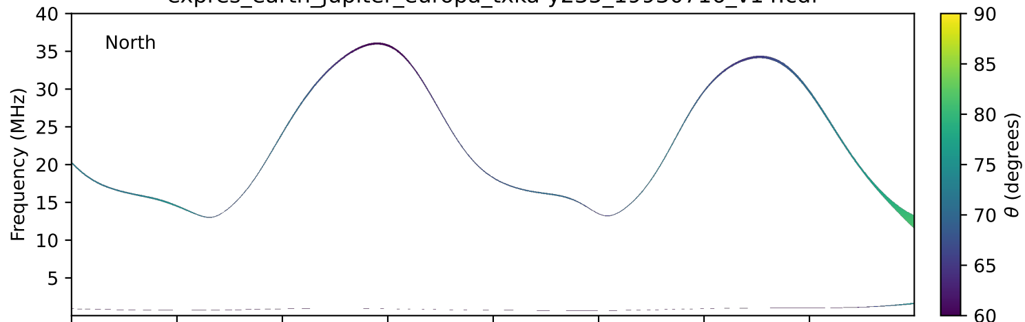
expres_earth_jupiter_europa_txka-y235_19930716_v14.cdf
